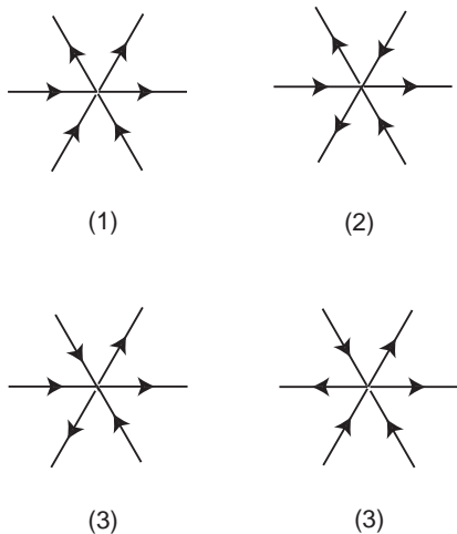
FIG. 11: Examples of three types of allowed vertices.
