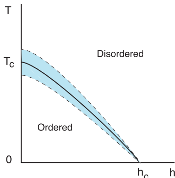
FIG. 9: Conventional phase diagram in which a finite temperature phase transition exists — the solid curve. The shaded region is the domain of classical critical fluctuations. The influence of the quantum critical point at h_c , at T = 0 , has to lie outside this domain.
