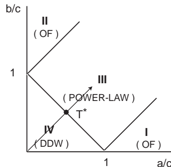
FIG. 4: The phase diagram. The regions I and II are orbital ferromagnets (OF). The region III is the power-law phase and the region IV is the orbital antiferromagnet with DDW order. The arrow marks a path (tetragonal symmetry assumed) from the low temperature to the high temperature phase with the pseudogap transition at T_c = T^* .
