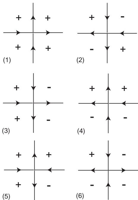
FIG. 6: The mapping of the first 6 vertices to equivalent spins on the dual lattice.
