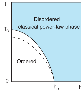
FIG. 10: The phase diagram in which the entire finite temperature disordered phase is a classical power-law phase — the shaded region. The dashed curve is the crossover scale for the classical critical fluctuations within the ordered phase. The quantum critical regime is entirely eliminated, except precisely at T = 0 . The ordered regime is under the influence of the stable broken symmetry fixed point.
