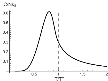
FIG. 5: The specific heat of the 6-vertex model as a function of T/T^* for a = b . Note that there are no observable anomalies at the transition at T^* , and the peak of the specific, which is entirely due to the analytic part of the free energy, is significantly below the transition.
