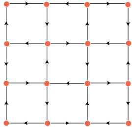
FIG. 1: A segment of the circulating current pattern in the DDW ordered state.
